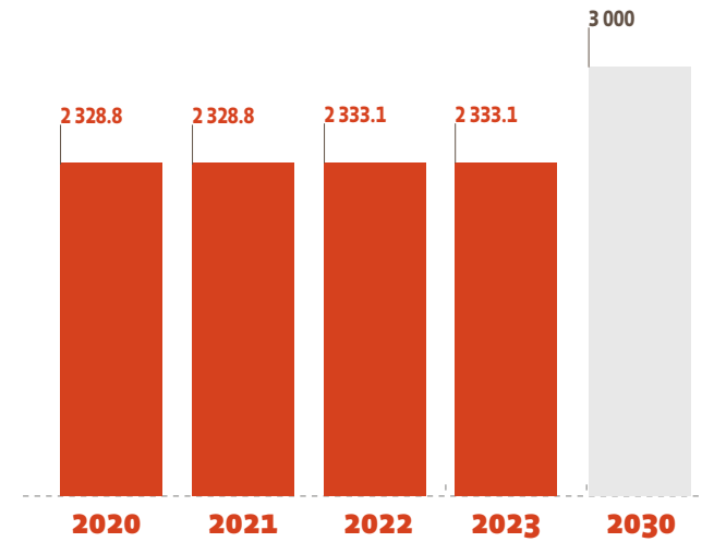
Source: EurObserv'ER
