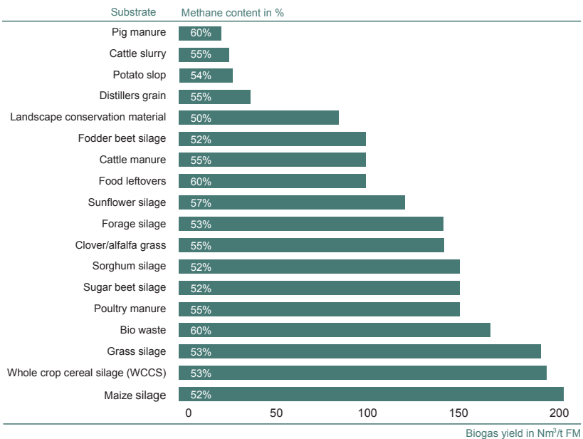
Figure 3.1.5.1: Biogas yield according to substrate in Nm³/t FM – FM means ‘fresh matter’. | Sources: FNR 2015, KTBL 2015. | Graphic: RENAC.
